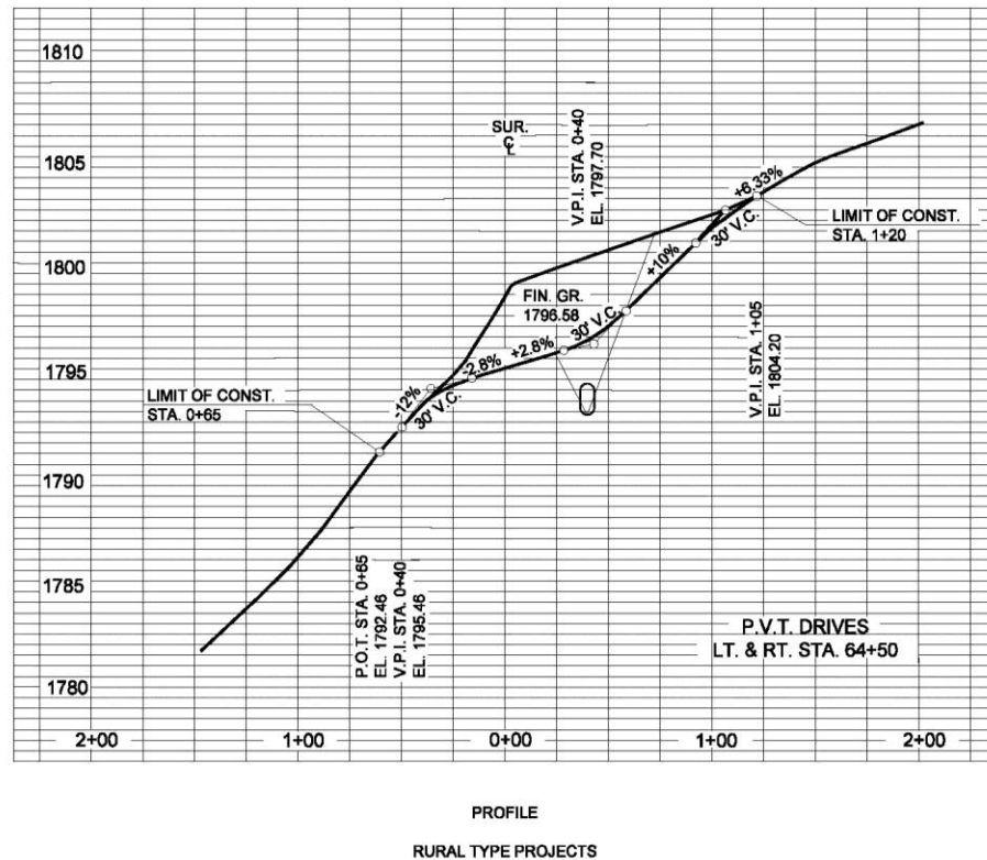
Figure 2-22 Rural Type Projects Typical Driveway Notation
