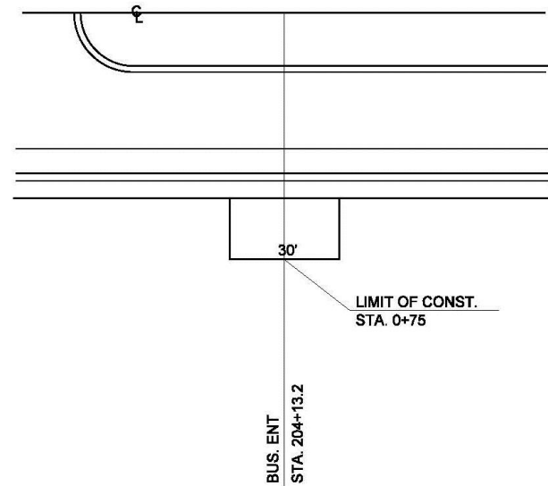
PROPOSED LAYOUT
