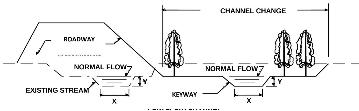
Figure 2-13 Channel Changes
